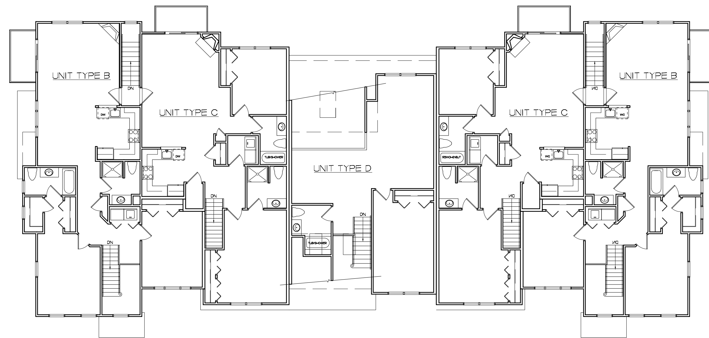
SECOND FLOOR - BUILDING 4 (7 UNITS)
